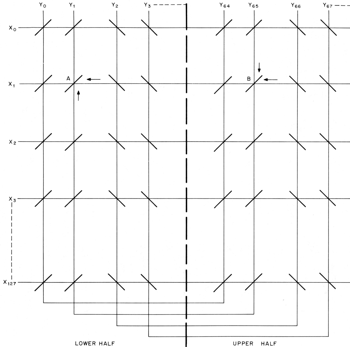
Figure 3-5 MM11-D Mat
