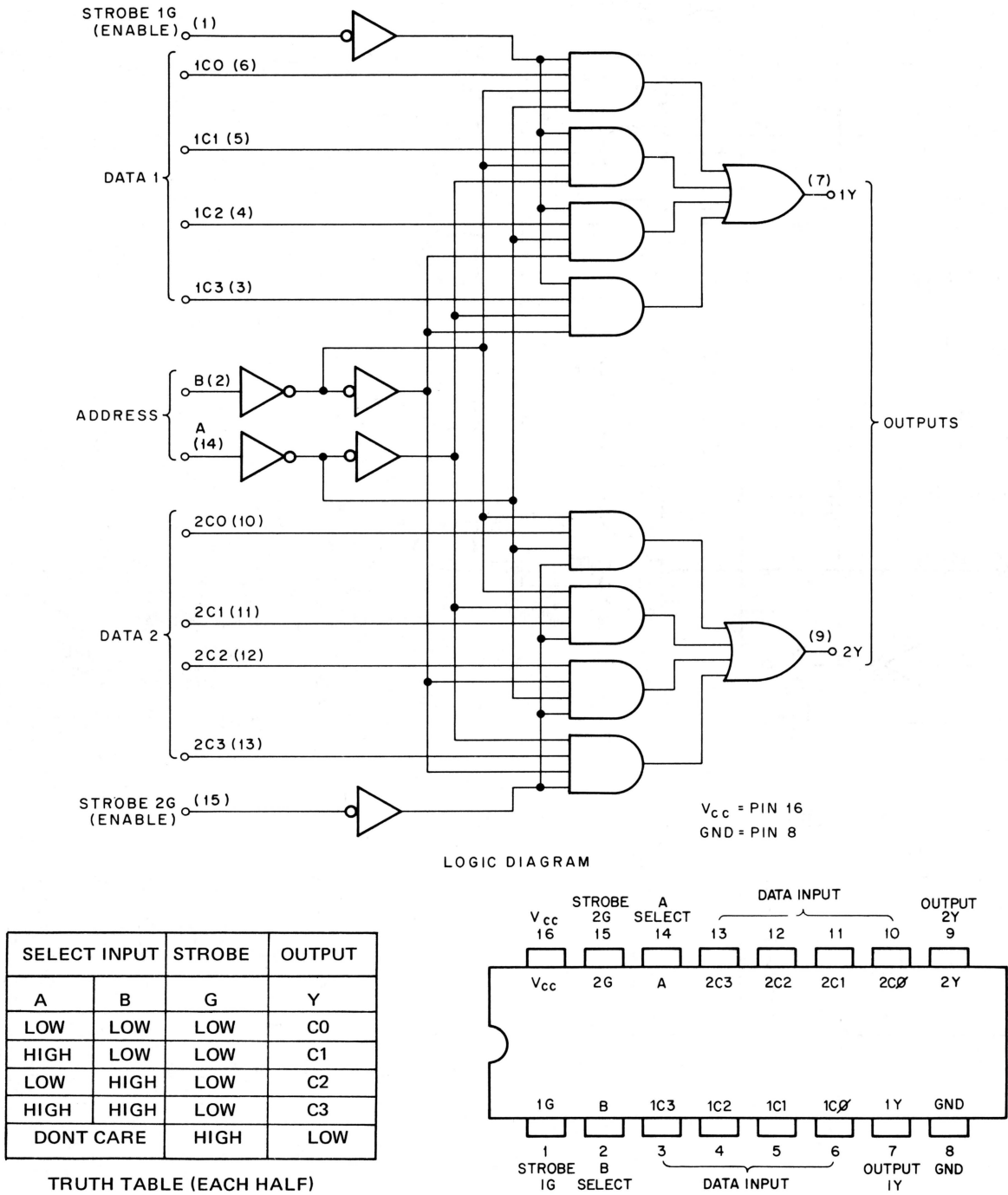
Figure A-6 74153
