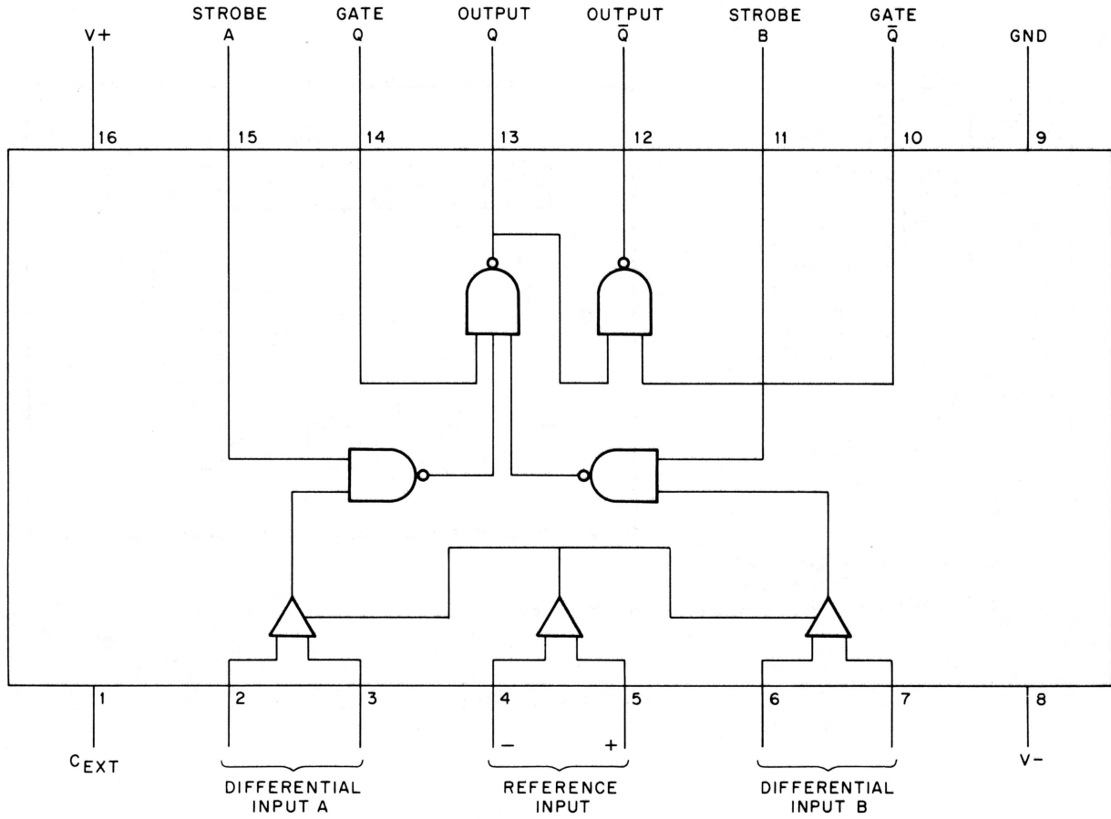
Figure A-4 7520
