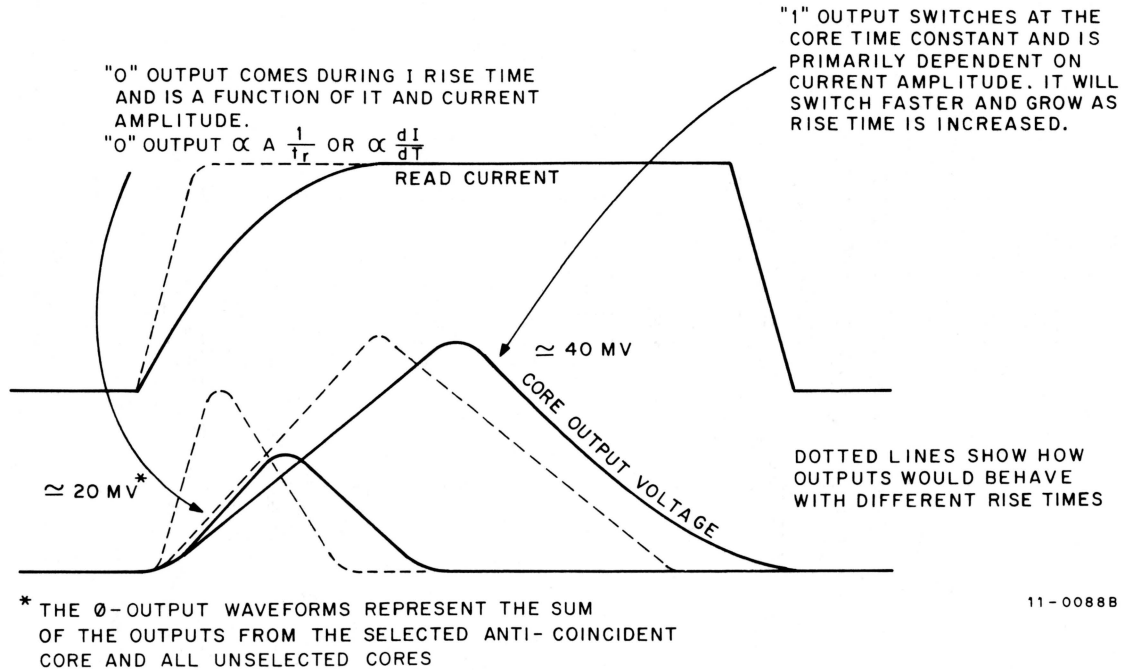
Figure 3-3 Core Current/Voltage Output Relationship
