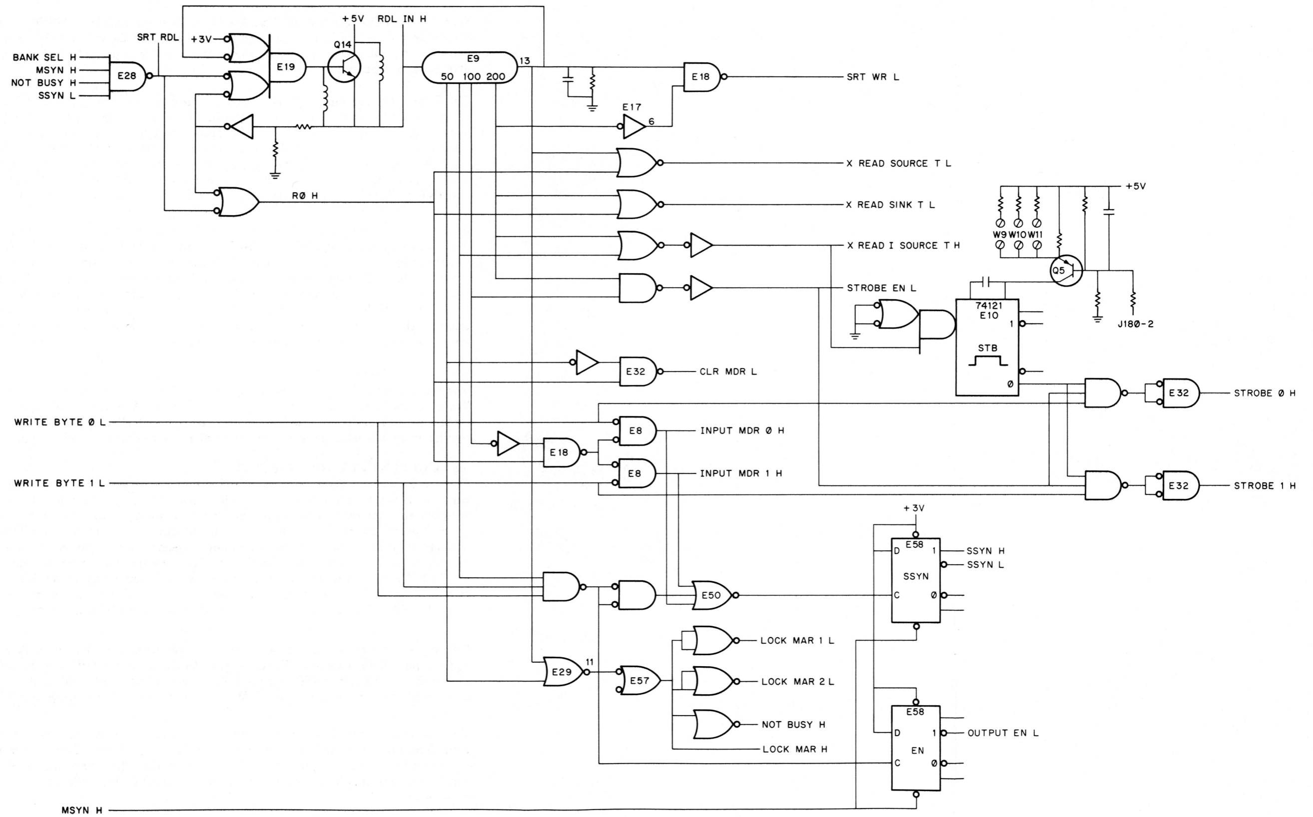
Figure 3-15 Read Control Logic
