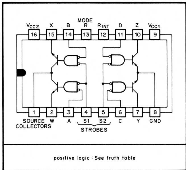
IC-75325
