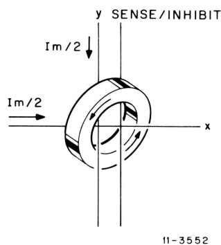
Figure 3-1 Core Windings
