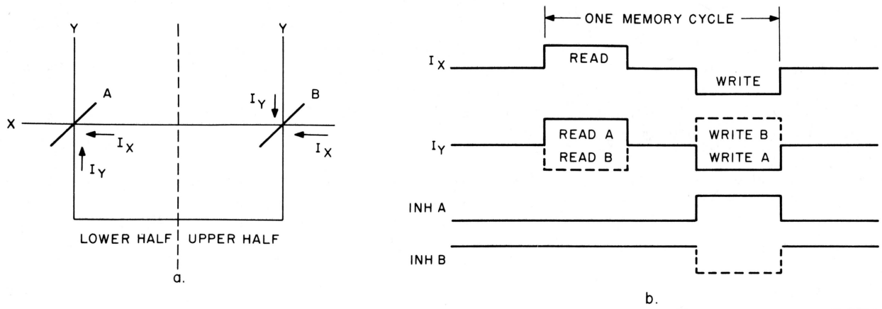
Figure 3-19 Phase Selection
