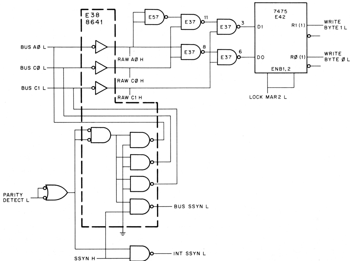
Figure 3-13 Control Bit Logic
