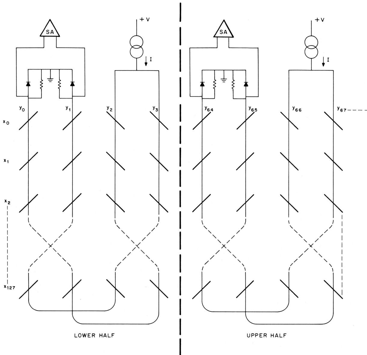
Figure 3-6 Mat Sense/Inhibit Windings
