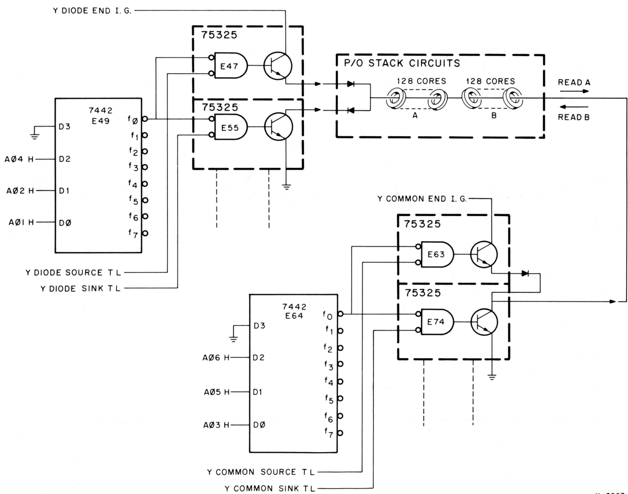
Figure 3-22 Y-Driver Circuit
