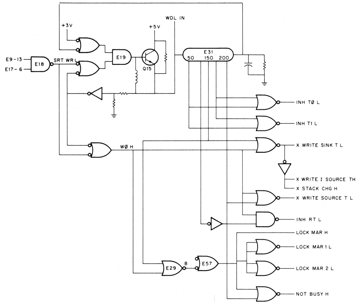
Figure 3-17 Write Control Logic
