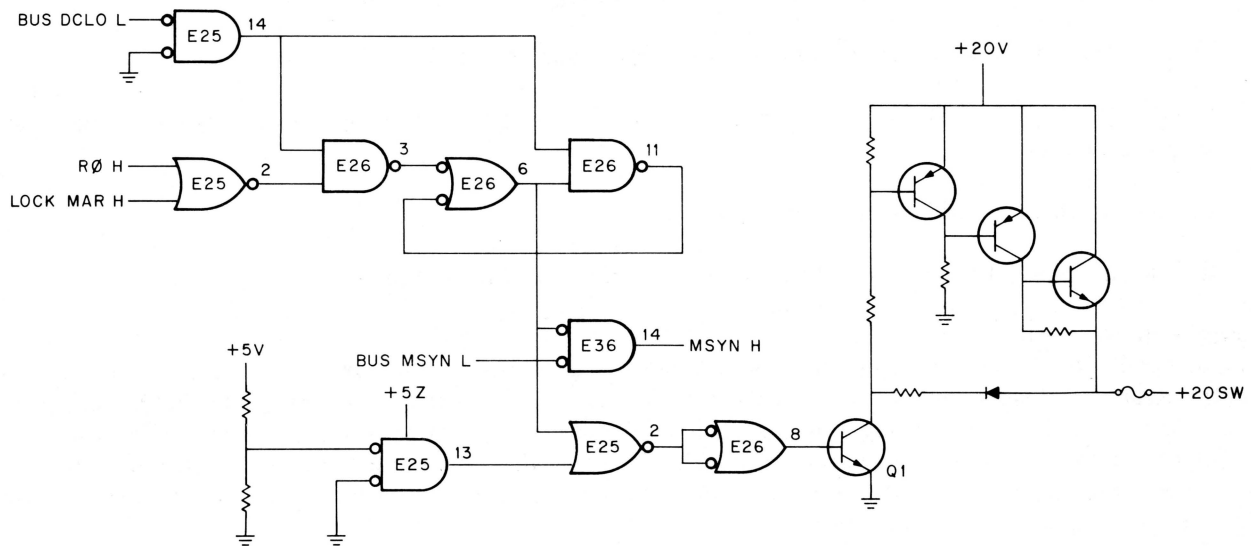
Figure 3-8 Voltage Monitor Circuit
