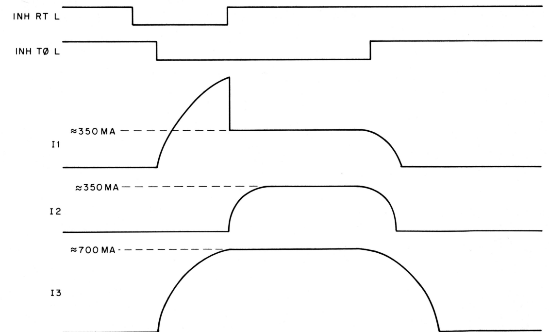
Figure 3-24 Inhibit Current Timing
