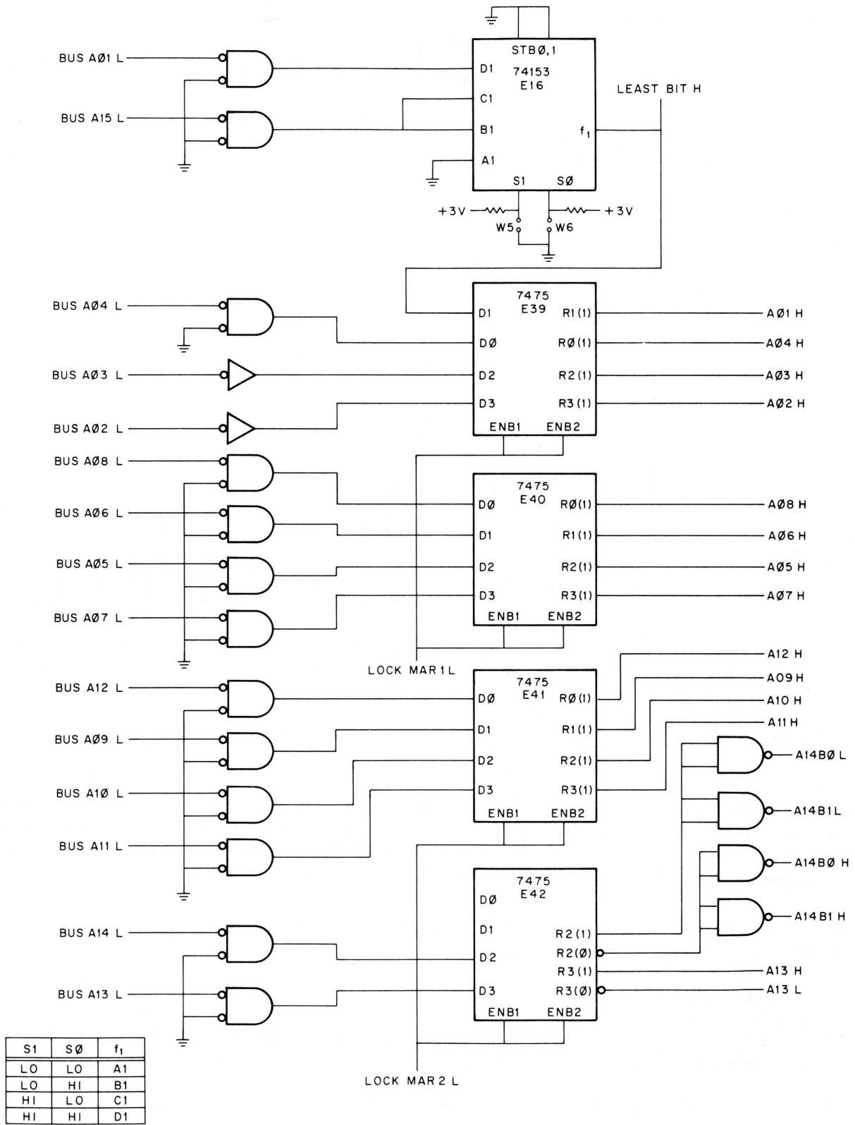
Figure 3-14 MAR Logic
