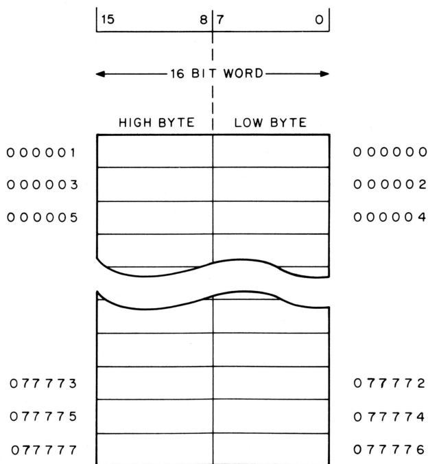
Figure 3-10 Memory Organization
