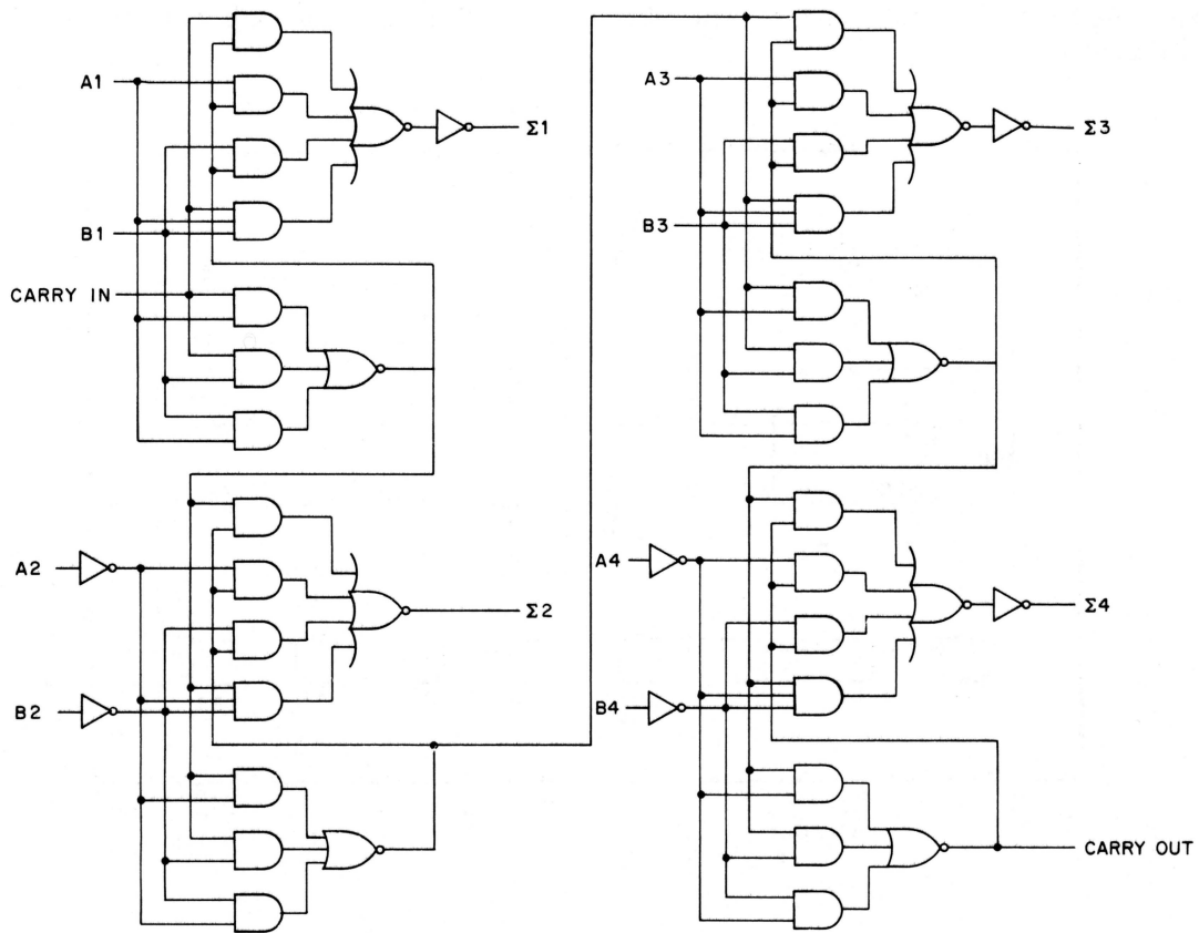
LOGIC DIAGRAM
